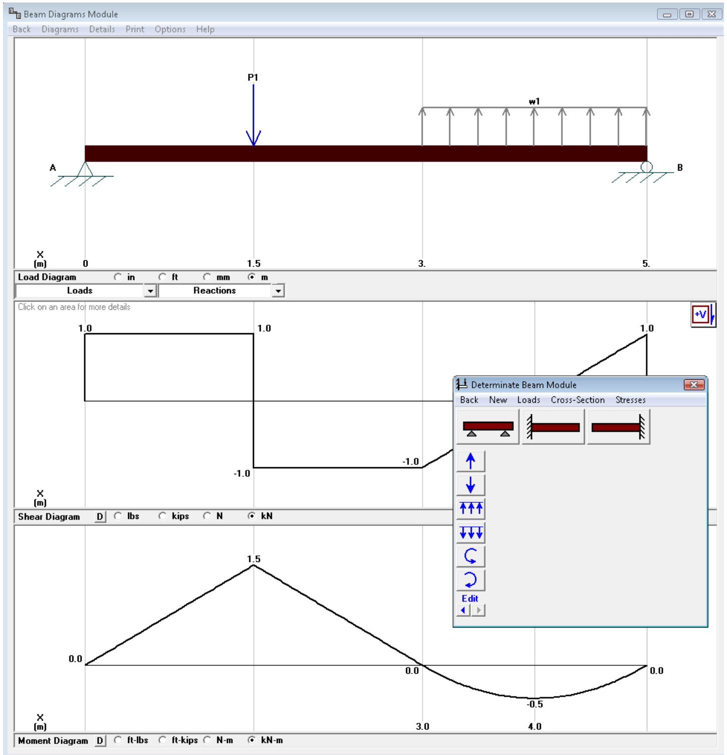
Screen image of usage of Determinate Beam Module of MDSolids
